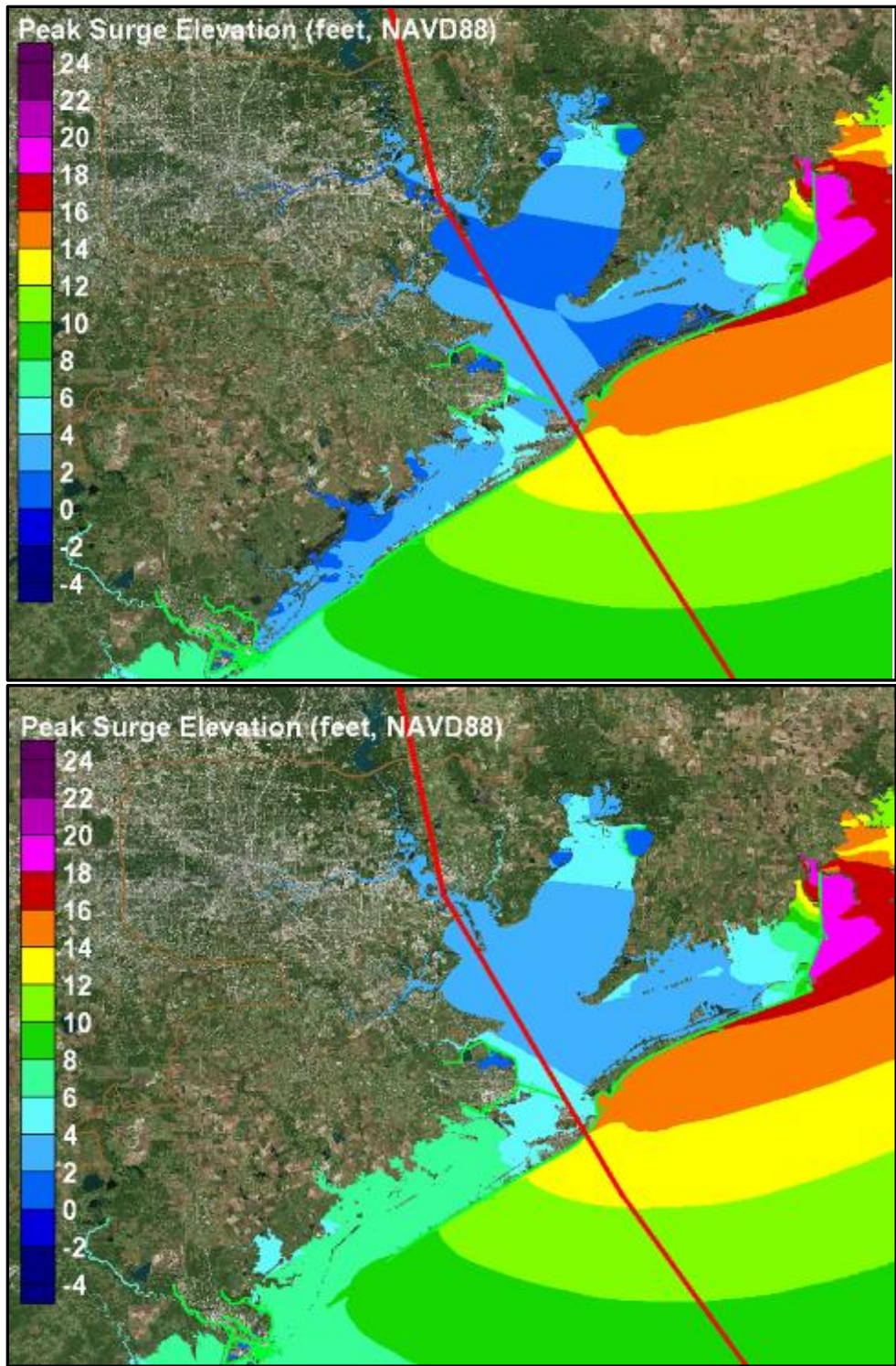
Figure 5. Peak Surge Maps for Hurricane Ike, Present Sea Level, for the Ike Dike Coastal Spine Concept Having a Western Section (top panel) and an Alignment Similar to the Likely USACE TSP that Does Not have a Western Section (bottom panel).
