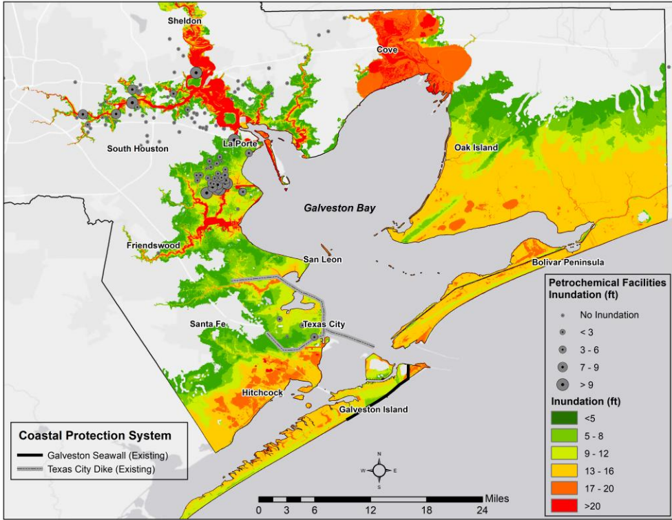
Figure 3: Petro and Chemical Plant Exposure to 500-year Inundation without Protection.
