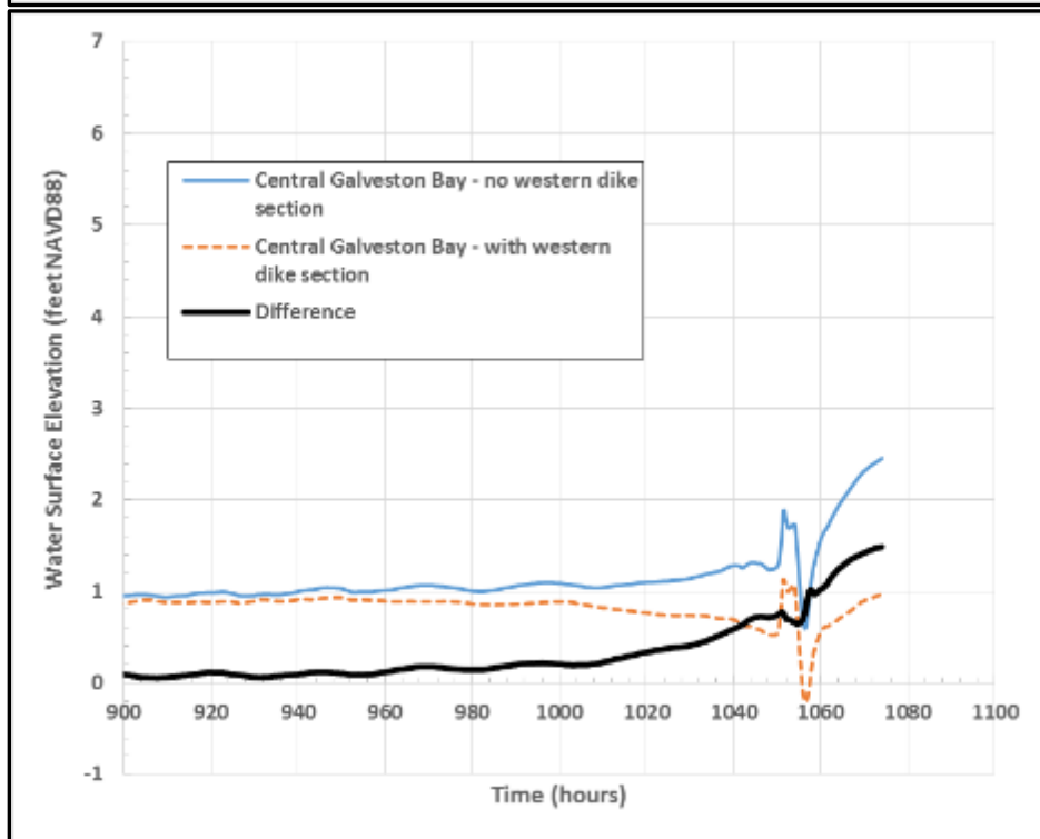
Figure 4. Water Surface Elevation in the Center of West Bay (Upper Panel) and Center Of Galveston Bay (Bottom Panel), With and Without a Western Section, for Hurricane Ike, Present Sea Level.
