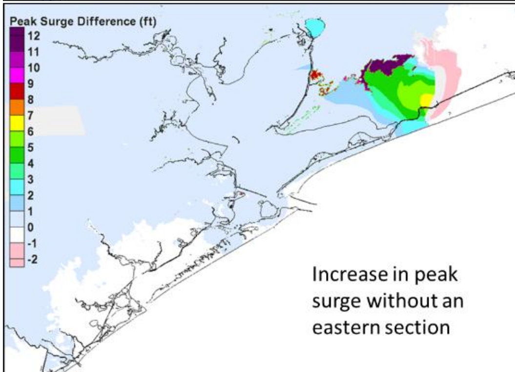
Figure 19. Increase in Peak Storm Surge Arising from Omission of the Western Dike Section (top panel), and Omission of the Eastern Dike Section, for Storm 033, Future Sea Level (bottom panel). Source: Authors.
