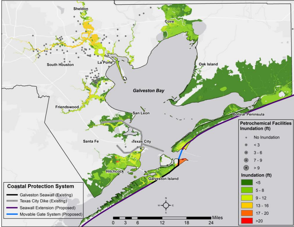
Figure 4: Petro and Chemical Plant Exposure to 500-year Inundation with Protection.
